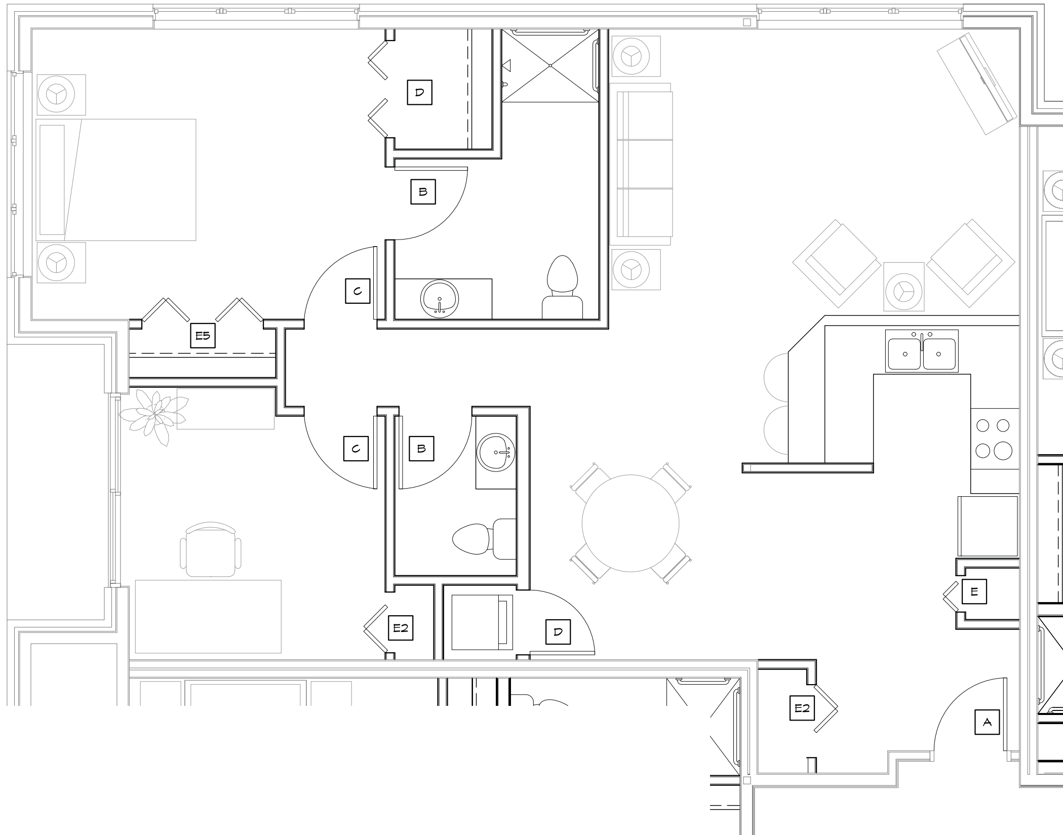
3 INDEPENDENT LIVING-TWO BEDROOM (UNIT 5) A2.4 1/4" = 1'-0"
